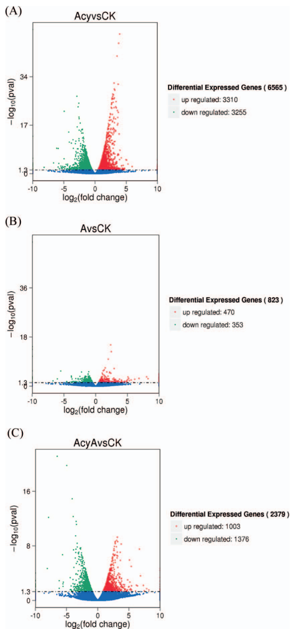
Fig. 2. Volcano plot of differentially expressed genes. (A) Volcano plot of differentially expressed genes after feeding by Acyrtosiphon gossypii (Acy). (B) Volcano plot of differentially expressed genes after feeding by Aphis gossypii (A). (C) Volcano plot of differentially expressed genes after feeding by both of Acyrtosiphon gossypii and Aphis gossypii (AcyA). Red dots indicate upregulated genes, green dots indicate downregulated genes ( P > 0.05 ), blue dots indicate nonsignificant genes ( P < 0.05 ).
