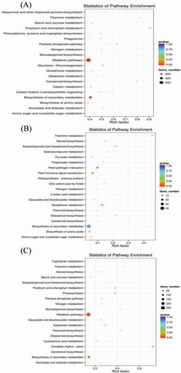
Fig. 6. Enrichment scatter plot of differential gene KEGG. (A) The differential gene KEGG in cotton was enriched feeding by Acyrtosiphon gossypii (Acy). (B) The differential gene KEGG in cotton was enriched feeding by Aphis gossypii (A). (C) The differential gene KEGG in cotton was enriched feeding by both of Acyrtosiphon gossypii and Aphis
