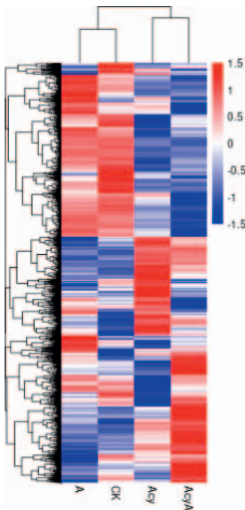
Fig. 3. Cluster analysis of differentially expressed genes in cotton after feeding by Acyrtosiphon gossypii (Acy) and/or Aphis gossypii (A). The \log_{10} (fragments per kilo base of exon per million reads [FPKM] + 1) value was normalized and transformed (scale number) and clustered. Red represented the high-expression gene, and blue represented the low-expression gene. Color from red to blue, representing \log_{10}(\text{FPKM} + 1) in descending order.
