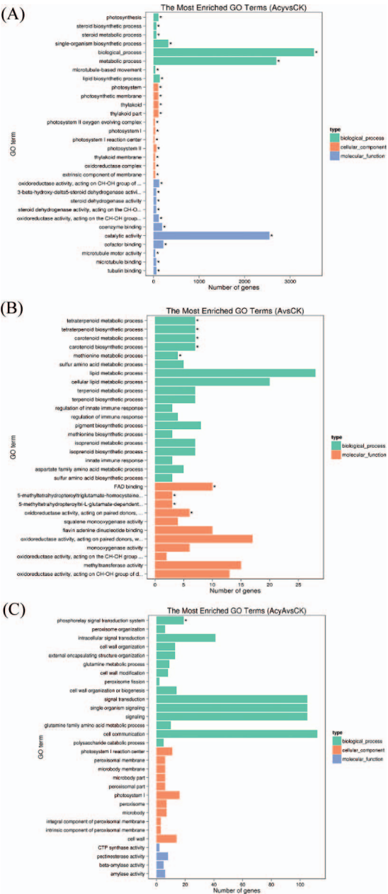
Fig. 5. Gene ontology (GO) enrichment column diagram. (A) GO enrichment analysis of cotton differentially expressed genes after feeding by Acyrtosiphon gossypii (Acy); (B) GO enrichment analysis of cotton differentially expressed genes after feeding by Aphis gossypii (A); (C) GO enrichment analysis of cotton differentially expressed genes after feeding by both of Acyrtosiphon gossypii and Aphis gossypii (AcyA). Different colors to distinguish biological processes, cellular components, and molecular functions. GOrms plot with “*” for significant enrichment.
