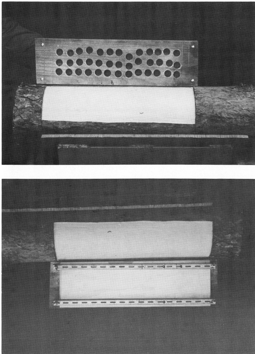
Fig. 1. a. Plywood front piece of sandwich showing pattern of holes, and b. reverse side with phloem under glass beside bolt from which section of bark and phloem has been stripped.
